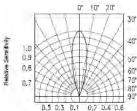
FIG.5 SENSITIVITY DIAGRAM
