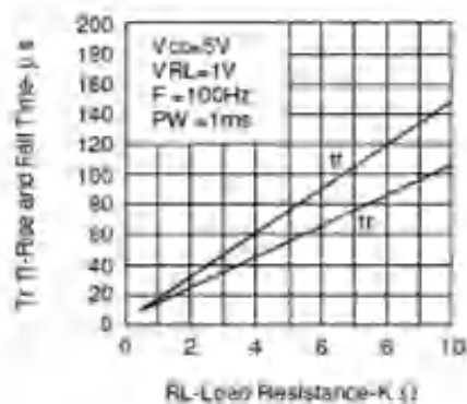
FIG.3 RISE AND FALL TIME VS LOAD RESISTANCE
