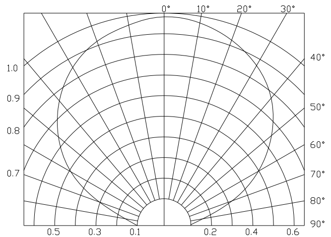
Radiation Diagram
