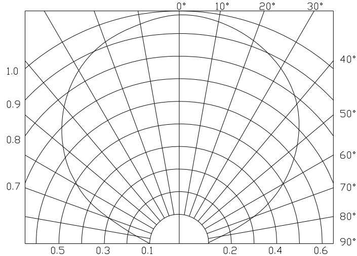
Radiation Diagram
