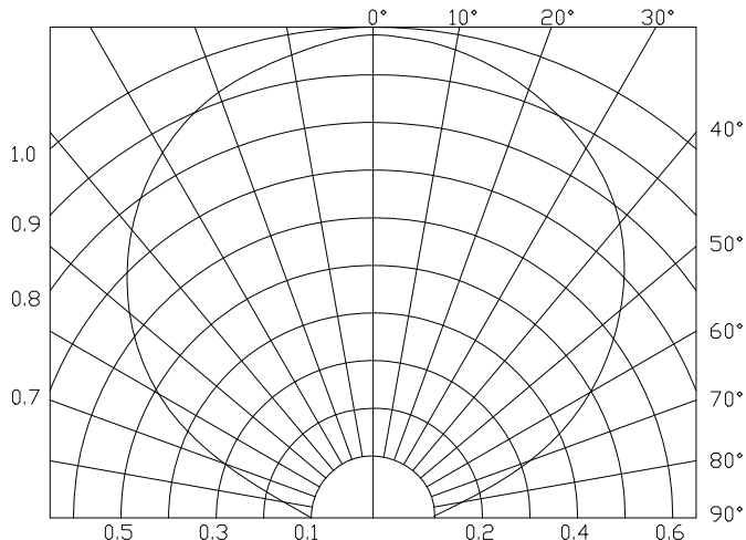
Radiation Diagram
