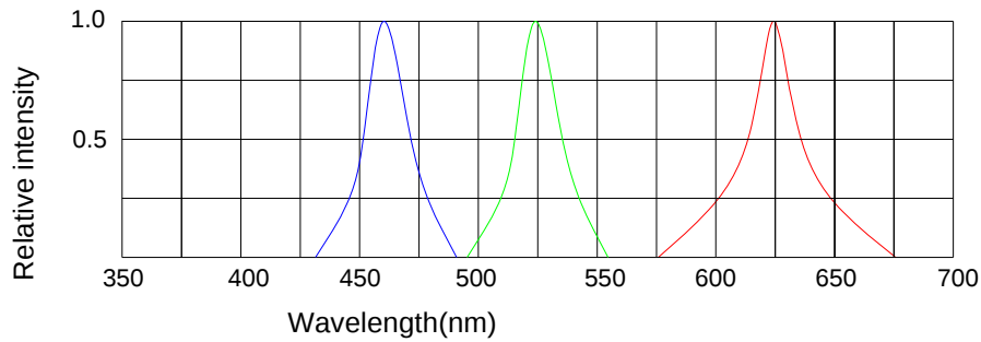
Wavelength Characteristics
