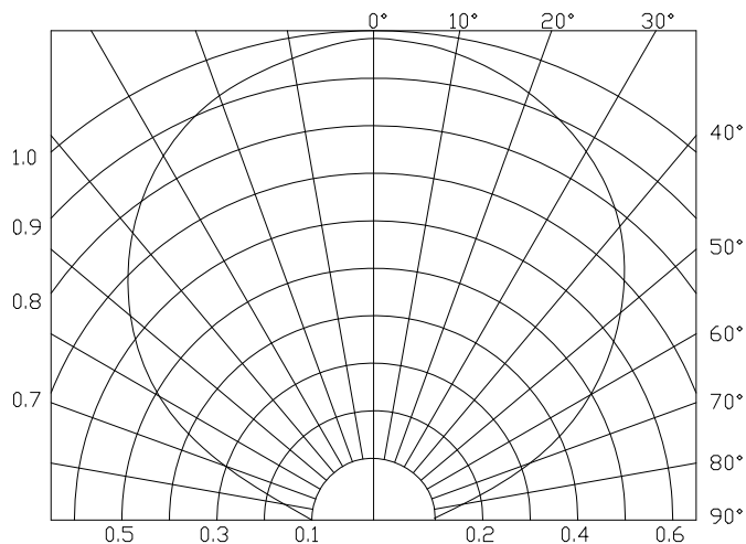
Radiation Diagram
